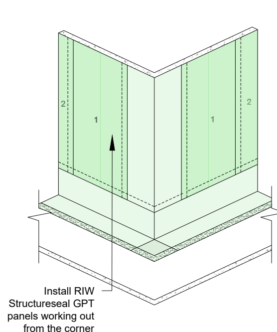
External Corner Stage 4
