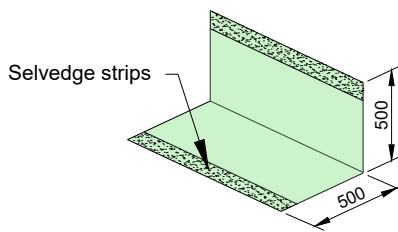
RIW Structureseal GPT Corner Strip
