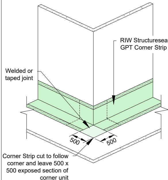
External Corner Stage 2
