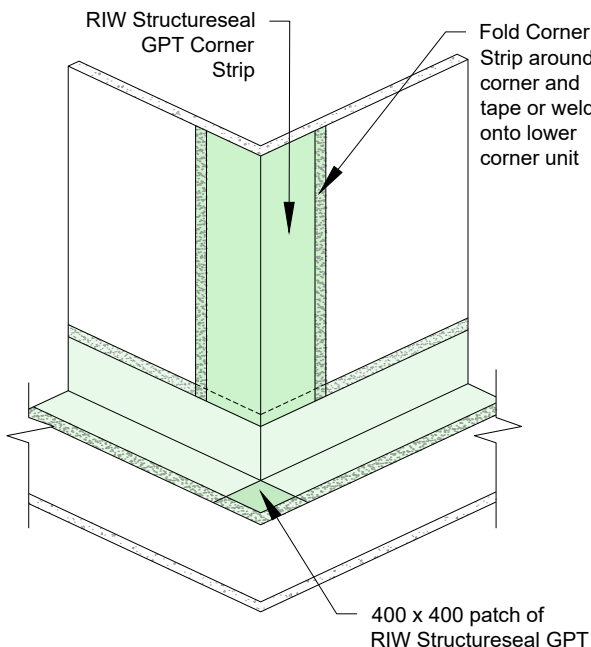
External Corner Stage 3
