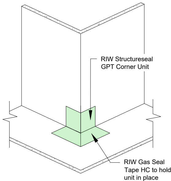
External Corner Stage 1
