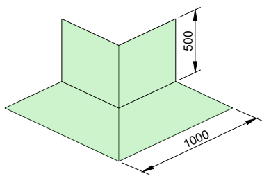
RIW Structureseal GPT External Corner
